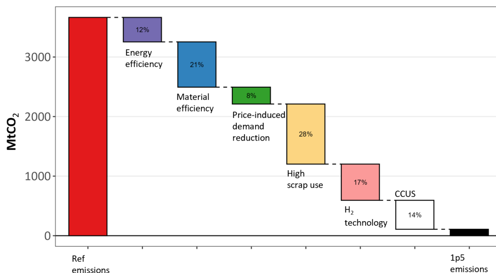
Figure 2. Contribution of different mitigation strategies to global steel emissions reductions by 2050, in a 1.5 °C-compatible scenario
